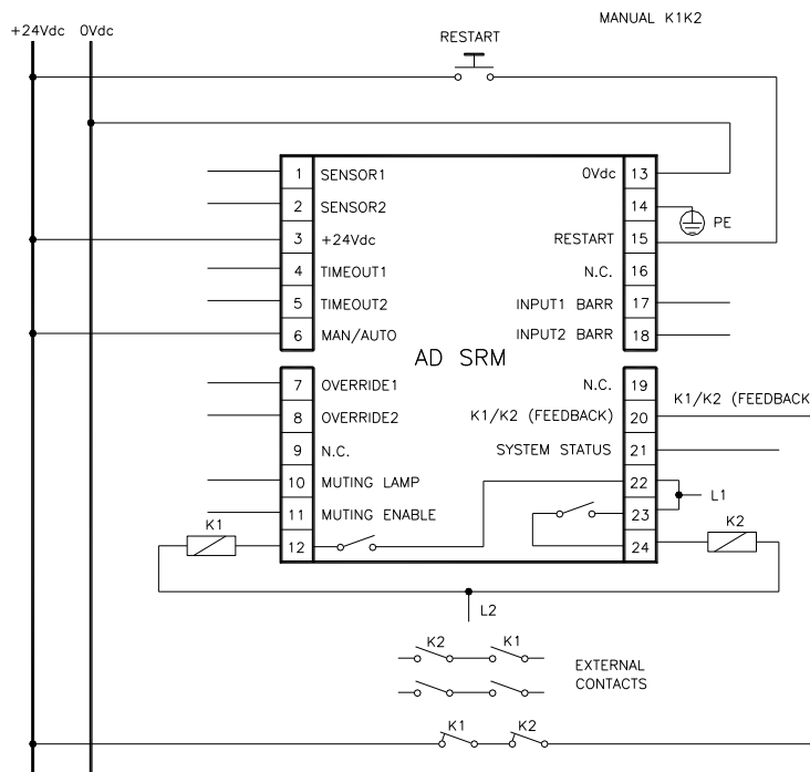
Figure 9 Manual operation with K1K2 relays
