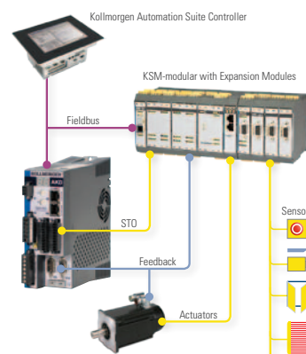
Example solution using the Kollmorgen Motion Safety concept.
