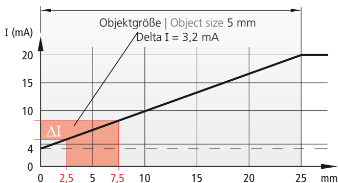
25 mm Messbereich | Measuring range
