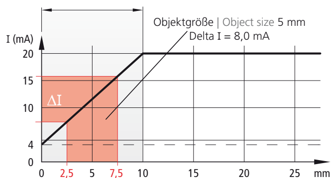
10 mm Messbereich | Measuring range
